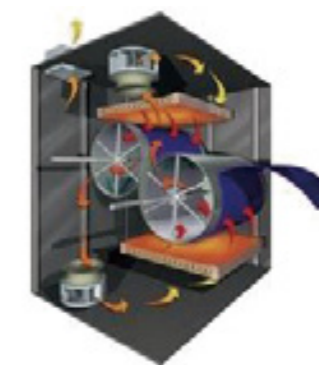
Through-Air Drum Drier Features Diagonally Offset Drums to increase Drying Area.
